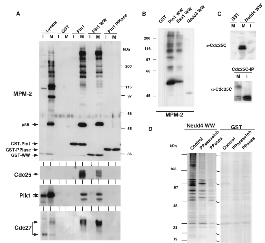
Fig. 1. Interaction between WW domains and subsets of phosphoproteins. (A) Interaction of the Pin1 WW domain and mitotic phosphoproteins. Interphase (I) and mitotic (M) HeLa cell lysates were incubated with glutathione beads containing control GST, GST-Pin1, its NH 2 -terminal WW domain, or COOH-terminal PPlase domain. After washing, proteins associated with the beads were subjected to immunoblotting analysis with MPM-2 antibody, or antibodies to specific proteins. Total lysates were used as control. (B) Interaction of WW domains and MPM2 antigens. GST or GST-WW domains of Pin1, Ess1, or Nedd4 were incubated with I or M HeLa extracts and washed. Bound proteins were detected with MPM-2. (C) Interaction between the Nedd4 WW domain and the mitotic Cdc25C in HeLa cells. (Top) Glutathione beads containing GST or GST-Nedd4 WW domain 2 were incubated with I or M HeLa cell extracts and washed. Immunoblotting analysis was done with antibodies to Cdc25C. (Bottom) Cdc25C immunoprecipitation (IP) and immunoblotting with the same antibodies as control. (D) Phosphorylation-dependent interaction between the Nedd4 WW domain and cellular proteins. Growing HeLa cells were incubated with [ 32 P]orthophosphate or 35 S-Met, and soluble proteins were subjected to GST-WW domain 2 pull-down assay before (control) or after treatment with three Ser-Thr phosphatases (PPases) in the absence or presence (Inh) of phosphatase inhibitors (19).
